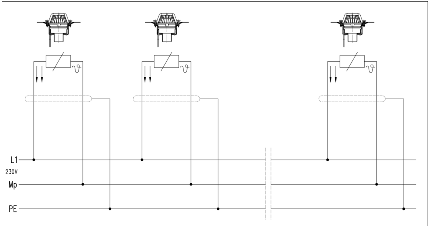
Illustration 10.61 Electrical connection diagram of the heating element
