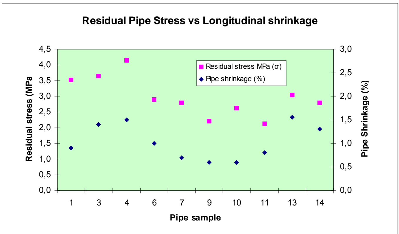
Illustration 2. Residual stress vs longitudinal shrinkage
