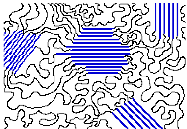
Illustration 1. Polyethylene molecules
