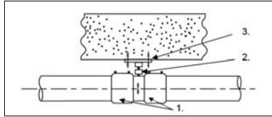
Illustration 8.1 Anchor bracket with 2 Akafusion couplers Art. Nr. 41xx95
